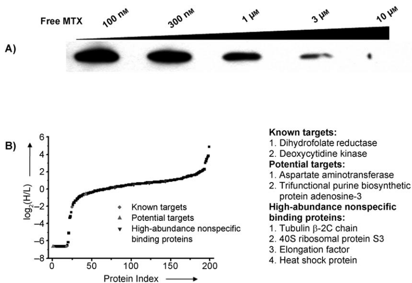
Figure 2. A) Western-blotting analysis of in vitro dendrimer–MTX targets with an anti-DHFR antibody. Free MTX was added at different concentrations as the competitive binding agent. B) Profiling of proteins identified in the SILAC experiment against their \log_2(H/L) value (H and L are the peak areas of the “heavy” and “light” peptides).
